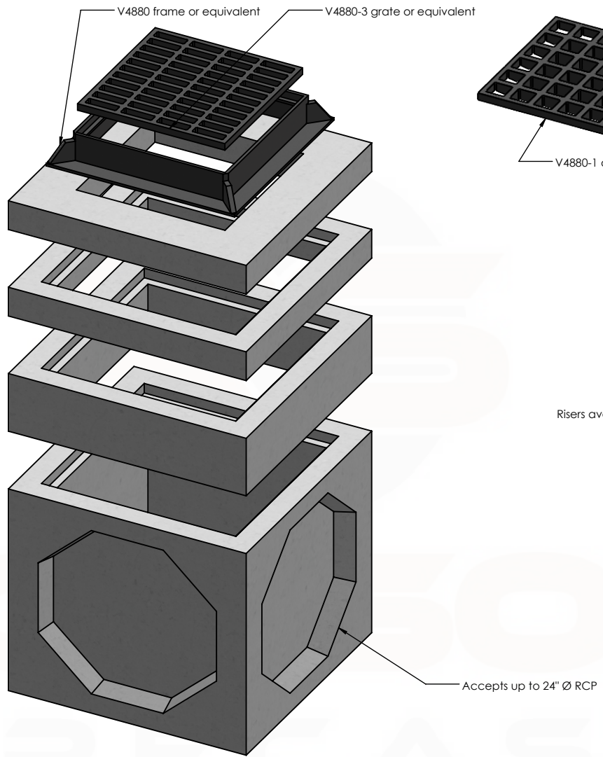
Exploded Isometric View Scale: 1/2' = 1'
