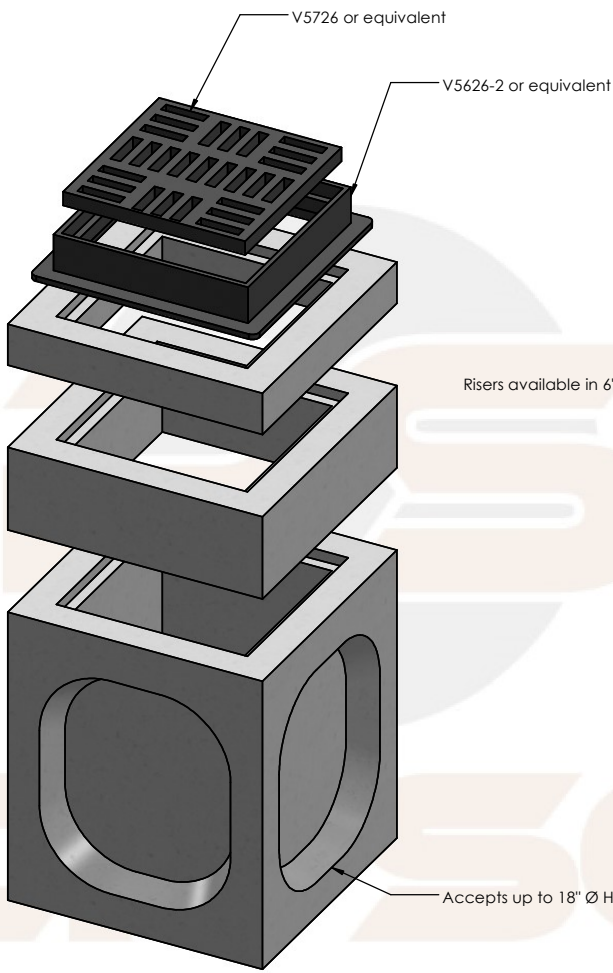
Exploded Isometric View Scale: 1/2" = 1'
